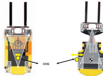
Counterbalance Forklift
